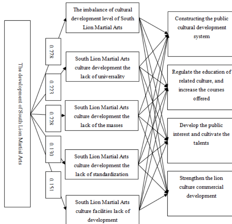
Figure 2. Computing results from the target layer to the scheme layer
